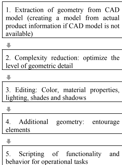
Figure 11. VR prototyping tool design process
